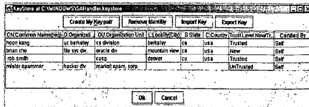
Figure 9: Key Store Manager
